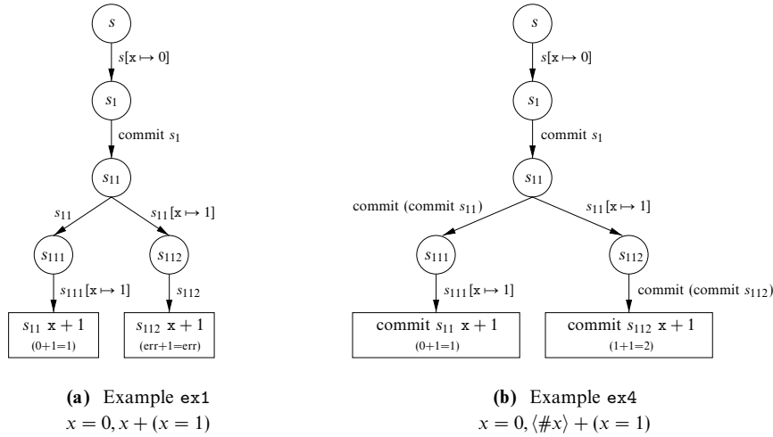
Fig. 2. Two examples of interleaving semantics with sequence points.
